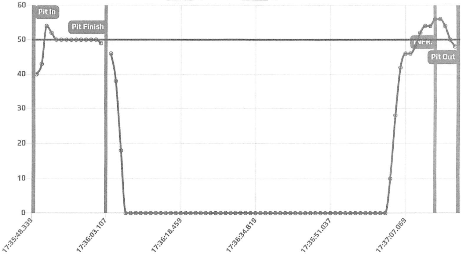
#36 GPS Speeds
